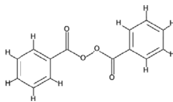
benzoyl peroxide
